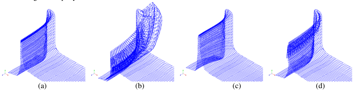
Fig. 6 Interface shape near the vertical tab in the profile die. (a) Substrate: LDPE-A, Cap: LDPE-A, (b) Substrate: LDPE-A, Cap: LDPE-D, (c) Substrate: LDPE-D, Cap: LDPE-A, (d) Substrate: LDPE-A, Cap: LDPE-A with larger flow rate (LFR) through the cap layer.
