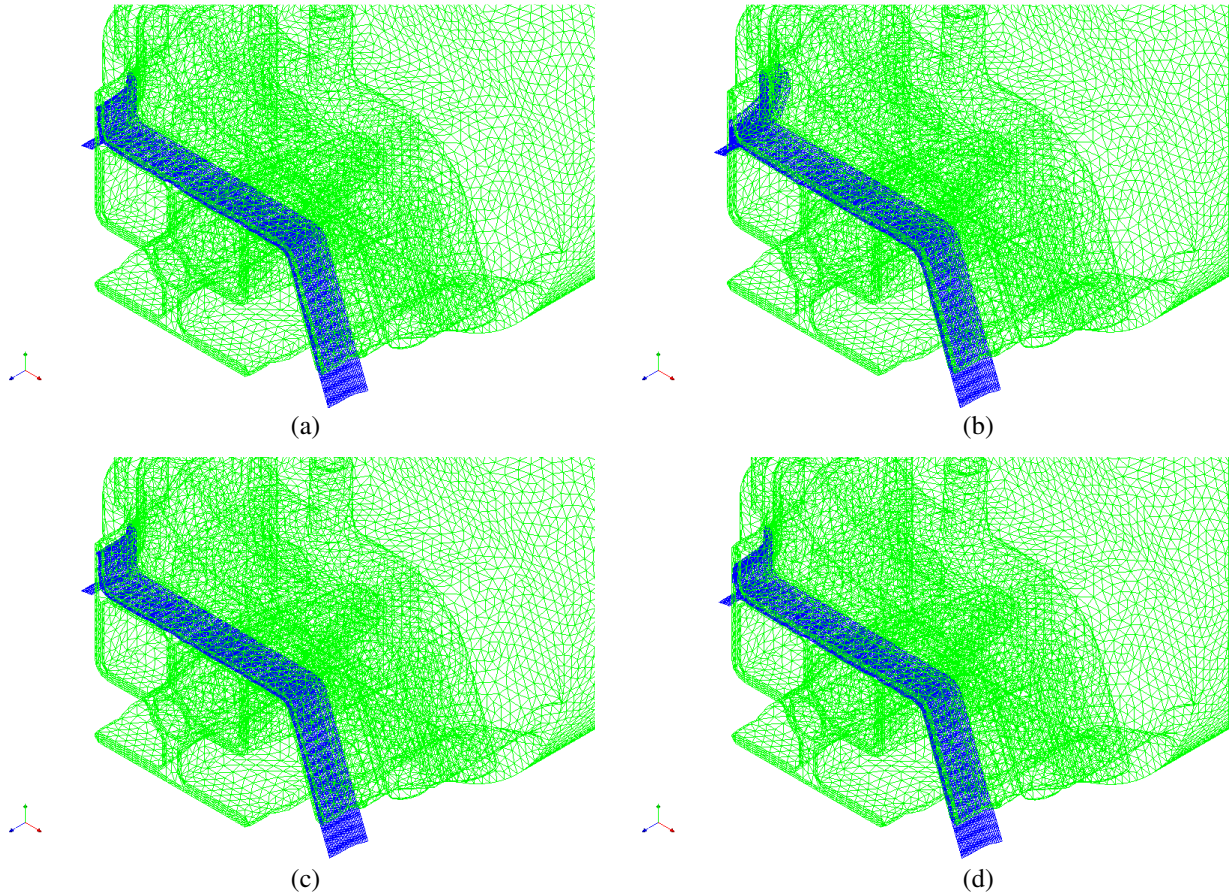
Fig. 5 Interface shape in the profile die. (a) Substrate: LDPE-A, Cap: LDPE-A, (b) Substrate: LDPE-A, Cap: LDPE-D, (c) Substrate: LDPE-D, Cap: LDPE-A, (d) Substrate: LDPE-A, Cap: LDPE-A with larger flow rate (LFR) through the cap layer.
