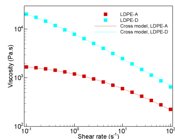
Fig. 2 Viscosity of two different grades of LDPEs [6].
