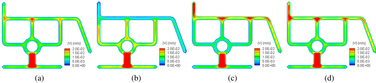
Fig. 8 Velocity distribution at the exit of the profile die. (a) Substrate: LDPE-A, Cap: LDPE-A, (b) Substrate: LDPE-A, Cap: LDPE-D, (c) Substrate: LDPE-D, Cap: LDPE-A, (d) Substrate: LDPE-A, Cap: LDPE-A with larger flow rate (LFR) through the cap layer.
