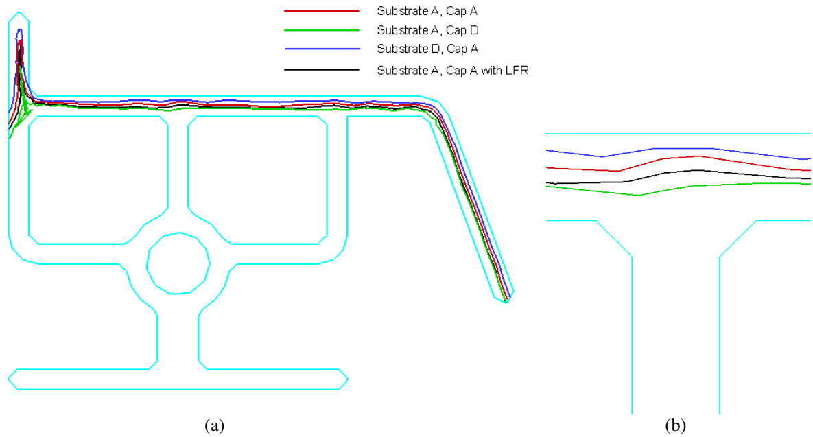
Fig. 7 Interface profiles at the exit of the profile die, (a) complete profile, (b) near the middle of the upper horizontal wall. (LFR: Larger Flow Rate in the cap layer)
