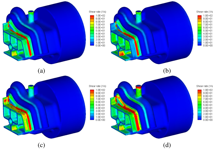
Fig. 11 Shear rate distribution in the profile die. (a) Substrate: LDPE-A, Cap: LDPE-A, (b) Substrate: LDPE-A, Cap: LDPE-D, (c) Substrate: LDPE-D, Cap: LDPE-A, (d) Substrate: LDPE-A, Cap: LDPE-A with larger flow rate (LFR) through the cap layer.
