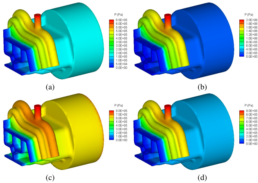
Fig. 10 Pressure distribution in the profile die. (a) Substrate: LDPE-A, Cap: LDPE-A, (b) Substrate: LDPE-A, Cap: LDPE-D, (c) Substrate: LDPE-D, Cap: LDPE-A, (d) Substrate: LDPE-A, Cap: LDPE-A with larger flow rate (LFR) through the cap layer.
