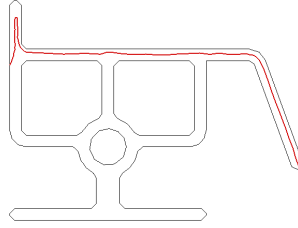
Fig. 4 Shape of the cap layer in the profile die. Interface between the cap layer and substrate is shown by red line.
