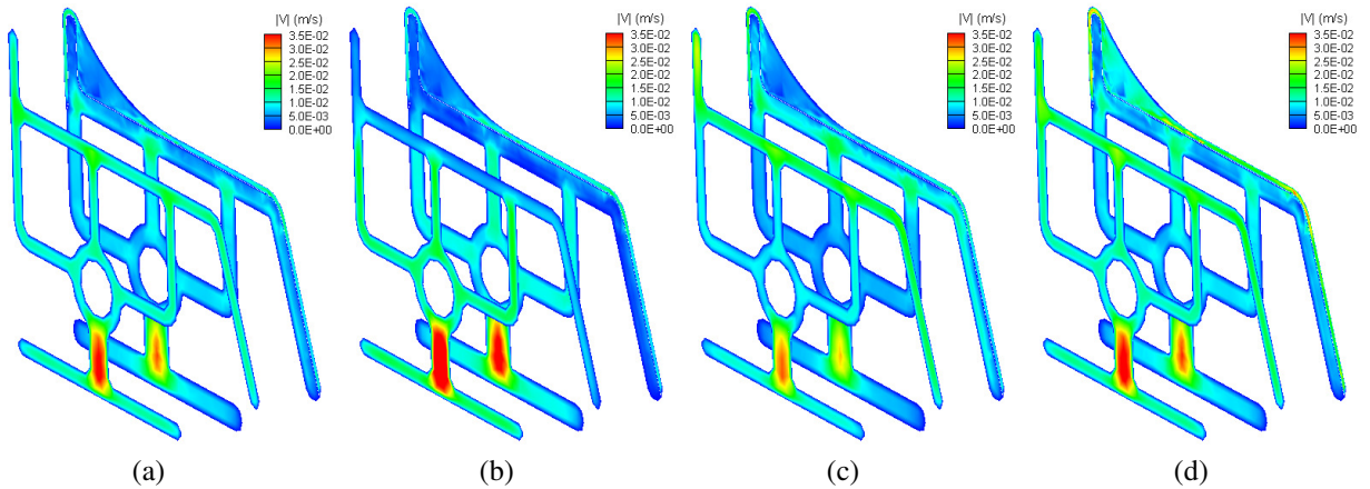
Fig. 9 Velocity distribution at the exit, and in the plane of the contact line of the profile die. (a) Substrate: LDPE-A, Cap: LDPE-A, (b) Substrate: LDPE-A, Cap: LDPE-D, (c) Substrate: LDPE-D, Cap: LDPE-A, (d) Substrate: LDPE-A, Cap: LDPE-A with larger flow rate (LFR) through the cap layer.
