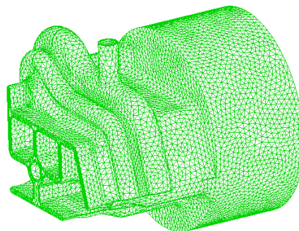
Fig. 3 Finite element mesh of tetrahedral elements in the profile die.
