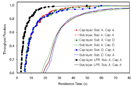
Fig. 12 Residence time distribution for the substrate and the cap layer of the profile die. (LFR: Larger Flow Rate in the cap layer)
